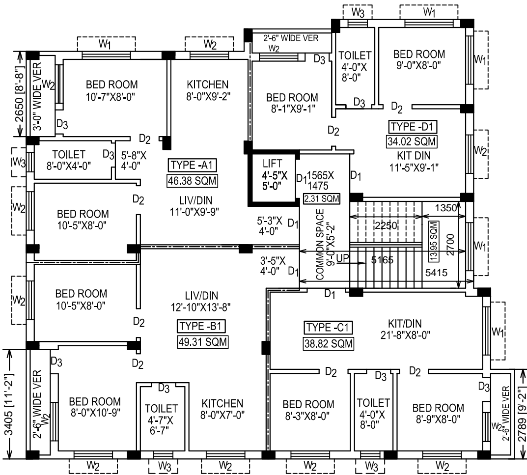
PRO. 1ST,FLOOR PLAN
